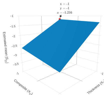
Fig. 4. Surface Plot: Composite-thickness combinations vs. |S_{21}|
