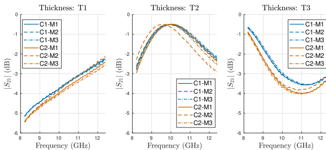
Fig. 1. |S_{21}| across different thickness configurations. Colors represent composite type, while line styles indicate mesh variation.
